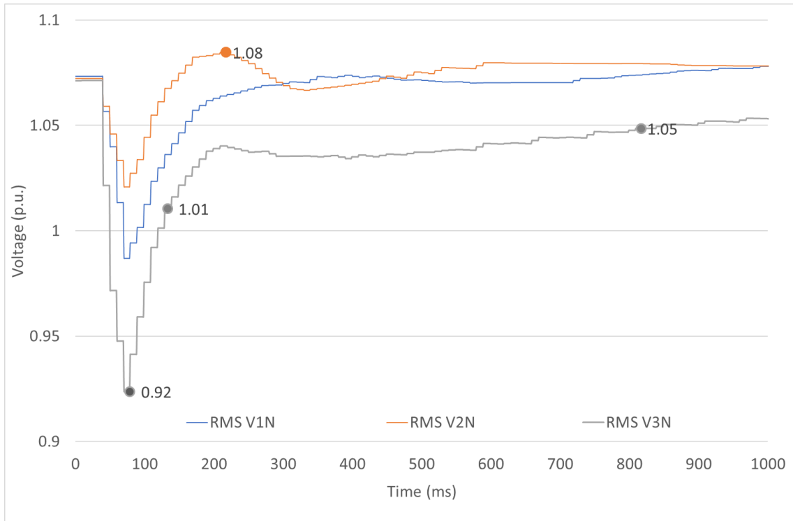
Figure 2: Demonstration of RMS Line-Neutral Voltages with Worst Case Highlighted
