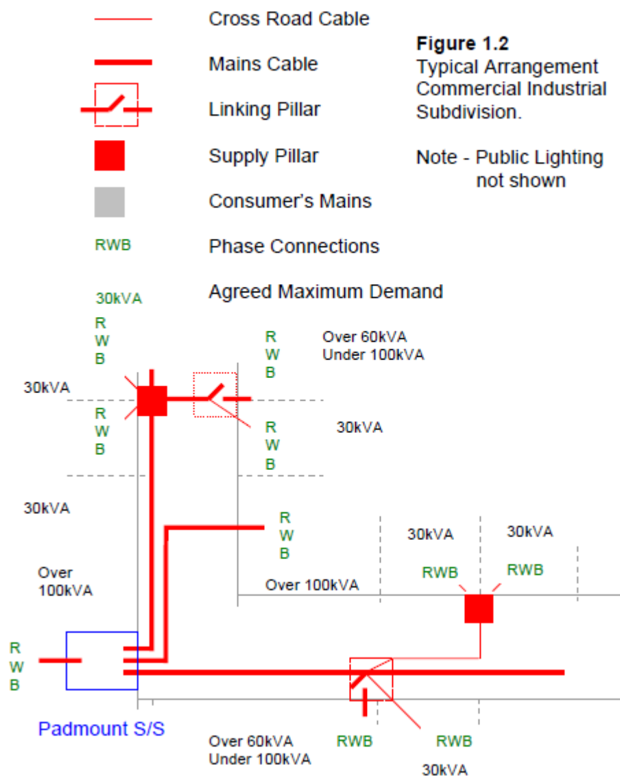
Figure 10 Typical arrangement Commercial / Industrial Subdivision
