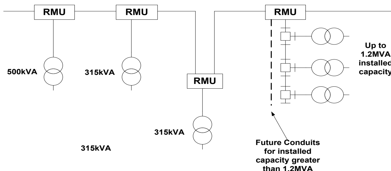
Figure 1 Radial Connection
