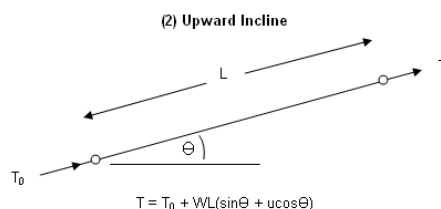
Figure 16 Upward Incline
