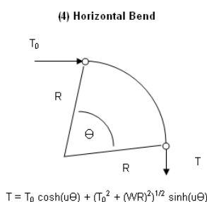
Figure 18 Horizontal Bend
