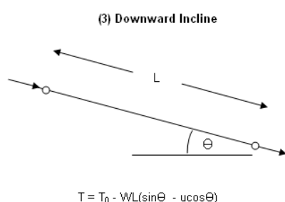
Figure 17 Downward Incline
