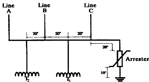
Figure C.2—An example of multilined two-transformer substation
