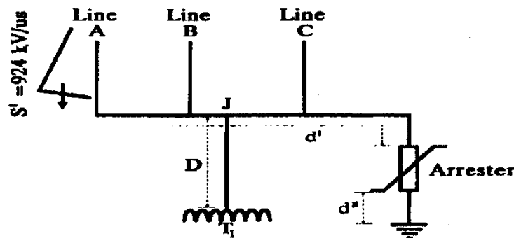
Figure C.3—Example 2—multilane two-transformer substation with an incoming surge on line A—transformer T2 not being considered is removed
