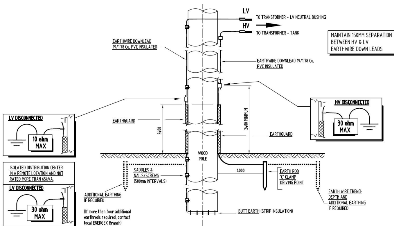
Figure 7: Pole Transformer with Separate Earthing System
