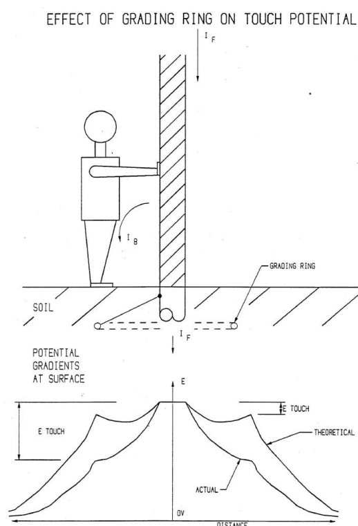
Figure 19: Grading Ring Reduction of Touch Potential
