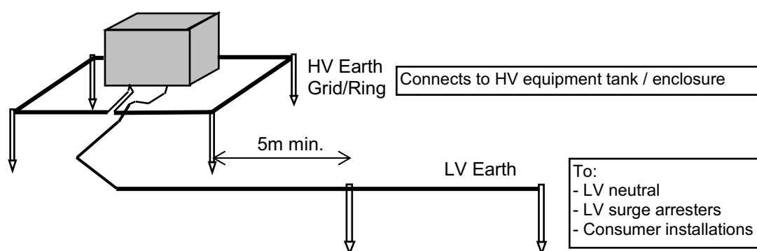
Figure 3: Typical Separate Earthing System for Overhead Network
