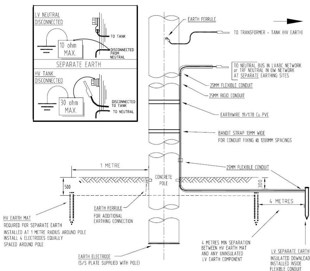
Figure 10: Conductive Pole with Separate Earthing
