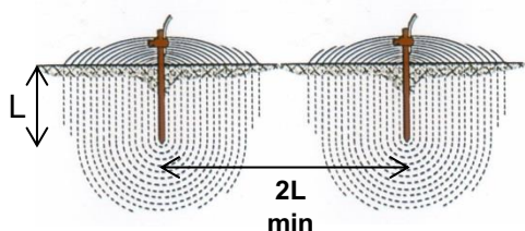
Figure 1: Horizontal Separation Between Electrodes
