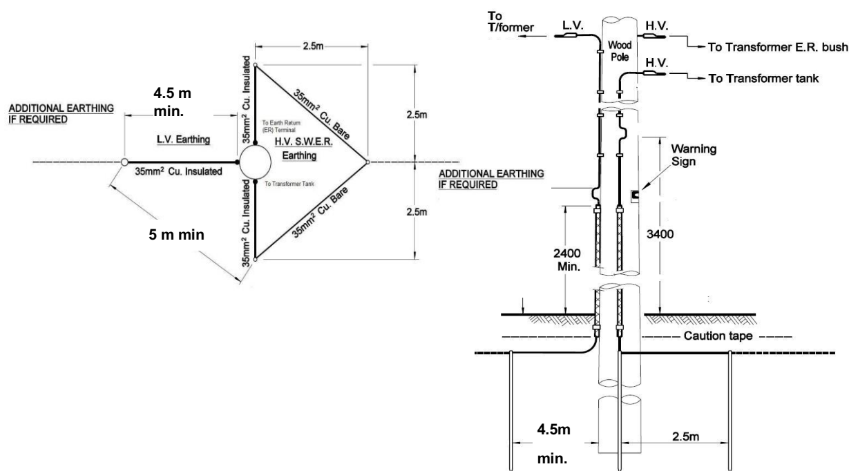
Figure 8: SWER Transformer Earthing
