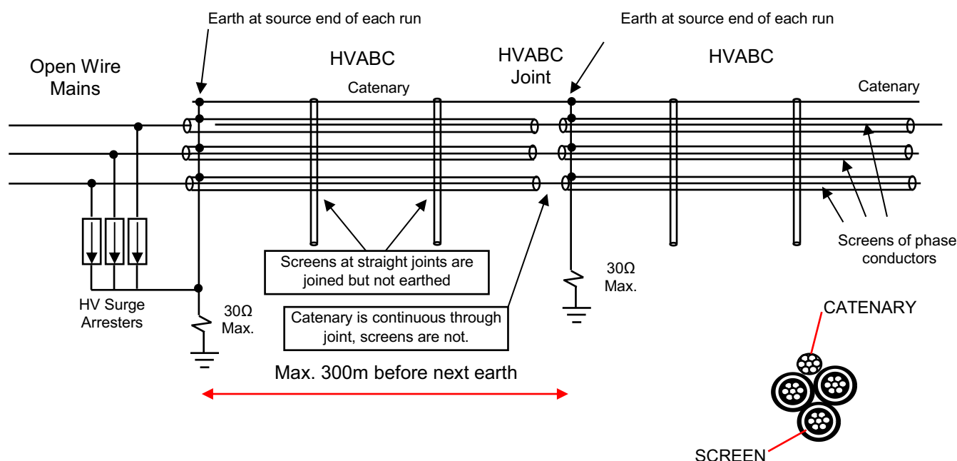
Figure 15: HV ABC Cable Earthing
